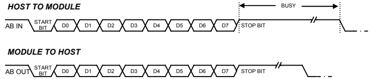
Fig1: Waveforms show TTL asynchronous serial, line 'A' follows TTL, line 'B' is inverted.
