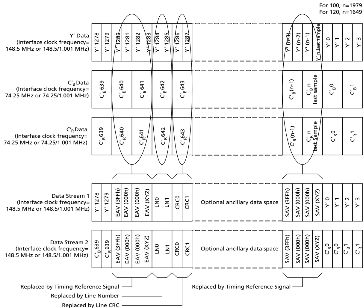
Figure 4-20: AviiA 20-bit Mapping Structure for 1280 x 720 100/120Hz Progressive 4:2:2 (Y'C'B'C'R) 8/10-bit Signals
