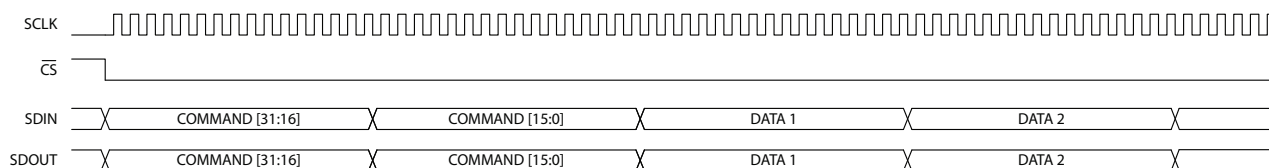
Figure 4-19: GSPI Write Timing – Auto-Increment
