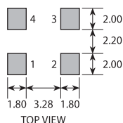
SOLDER PAD LAYOUTS
