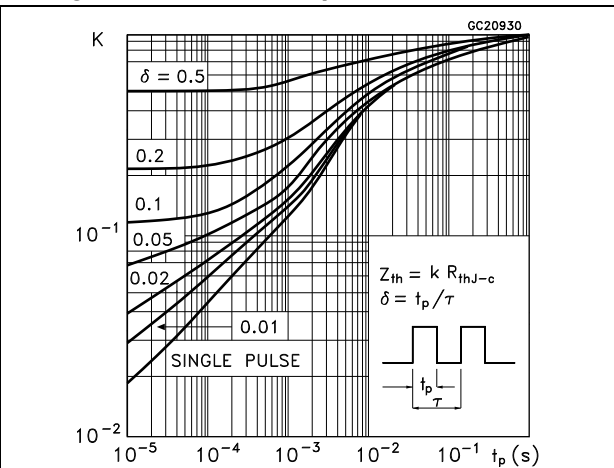
Figure 15. Thermal impedance for TO-247
