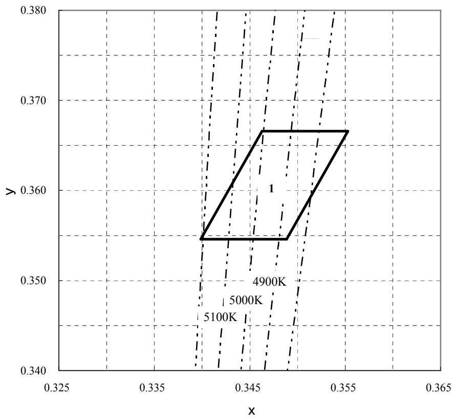
Chromaticity Diagram
