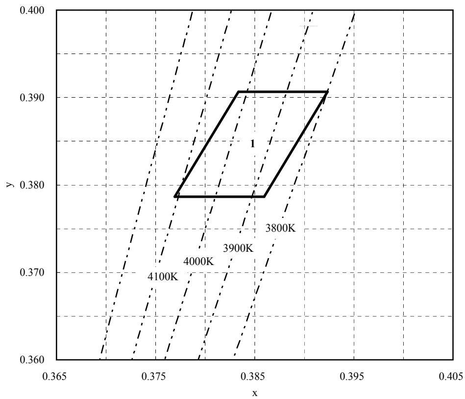
Chromaticity Diagram
