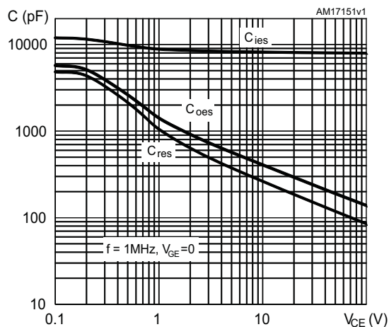
Figure 14. Capacitance variations
