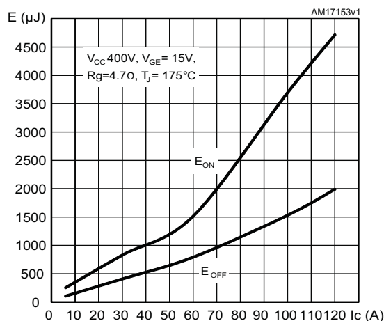
Figure 16. Switching energy vs. collector current
