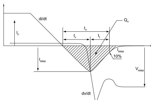
Figure 31. Diode recovery time waveform
