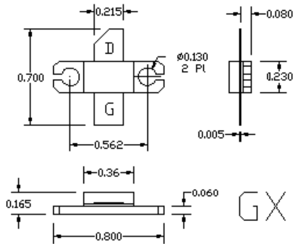
PACKAGE DIMENSIONS IN INCHES
