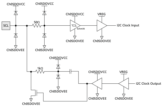
Figure 6-8: I 2 C, SCL, SDA
