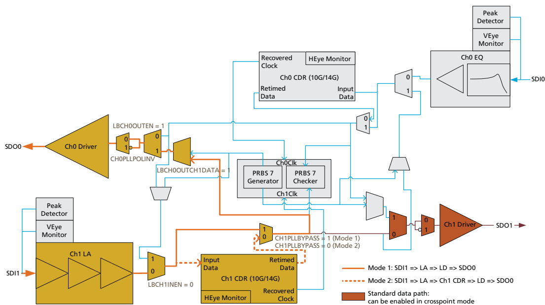
Figure 3-6: Crosspoint Modes 1 & 2
