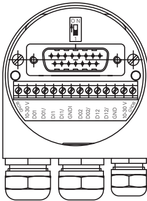
Arriving interface (male connector)
