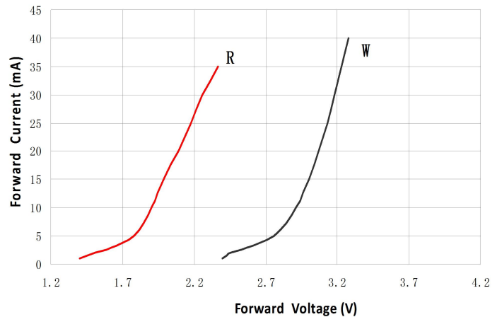
Forward Current VS. Forward Voltag (Ta=25°C)
