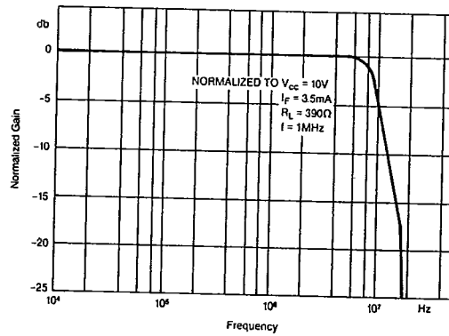
H11V GAIN ROLLOFF
