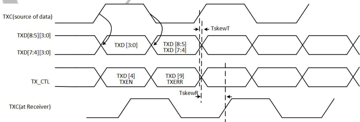
Figure 5-9 RGMII Interface Transmit Timing
