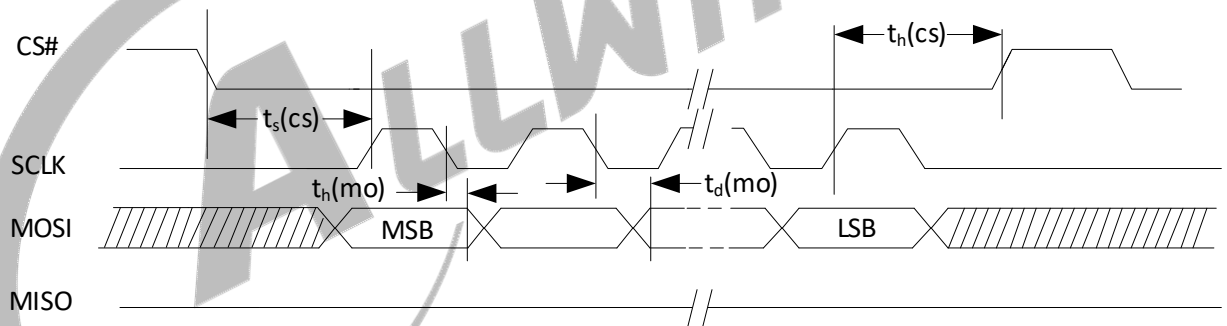
Figure 5-13 SPI Writing Timing
