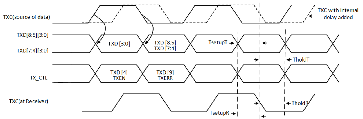
Figure 5-12 RGMII-ID Interface Receive Timing
