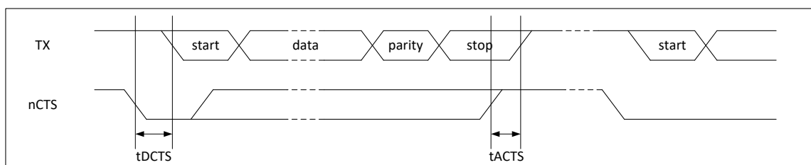
Figure 5-18 UART nCTS Timing
