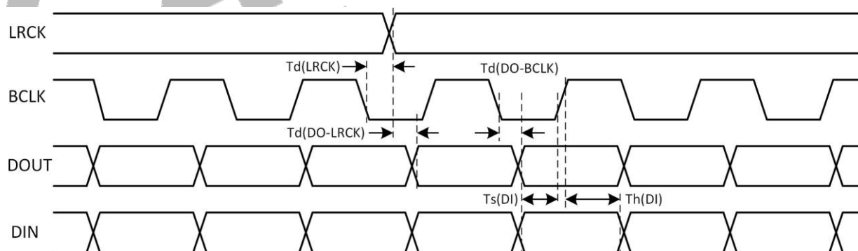
Figure 5-21 I2S/PCM Timing in Master Mode
