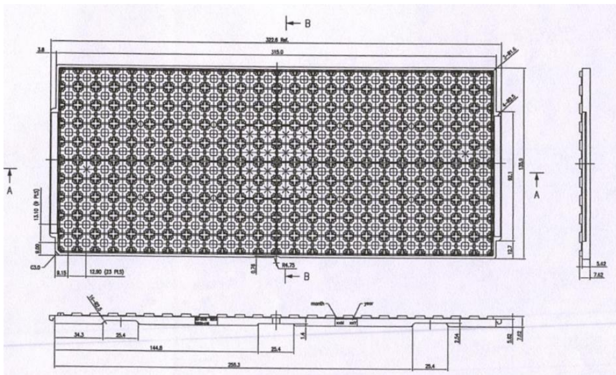
Figure 8-1 H133 Tray Dimension Drawing
