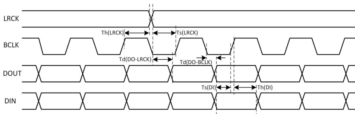
Figure 5-22 I2S/PCM Timing in Slave Mode
