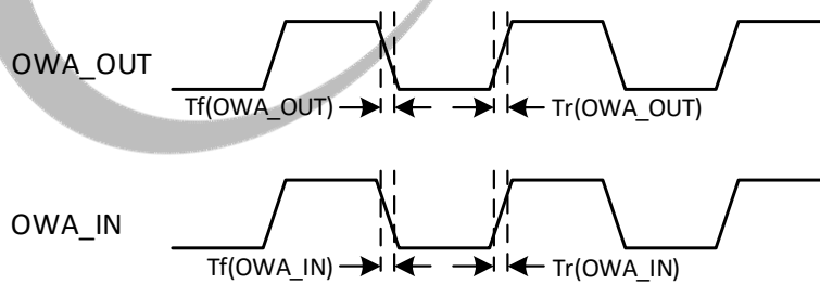
Figure 5-24 OWA Timing
