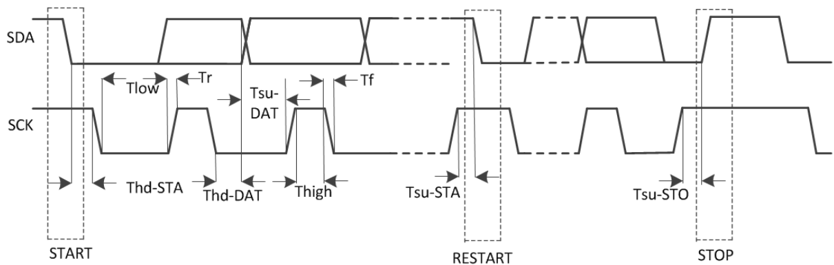
Figure 5-20 TWI Timing
