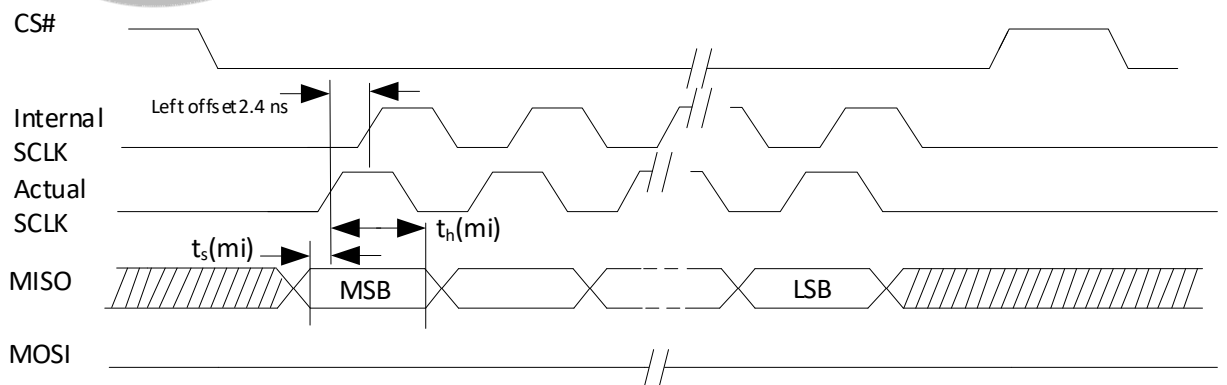
Figure 5-14 SPI Reading Timing
