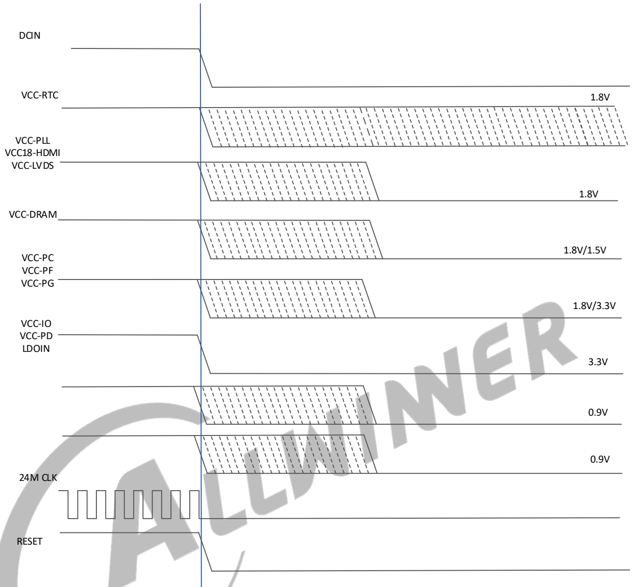
Figure 5-27 Power-Off Timing
