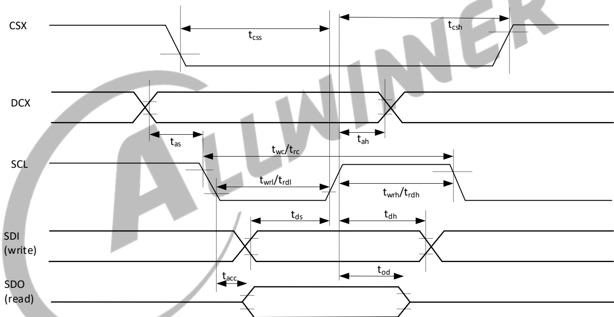
Figure 5-16 DBI 4-line Serial Interface Timing
