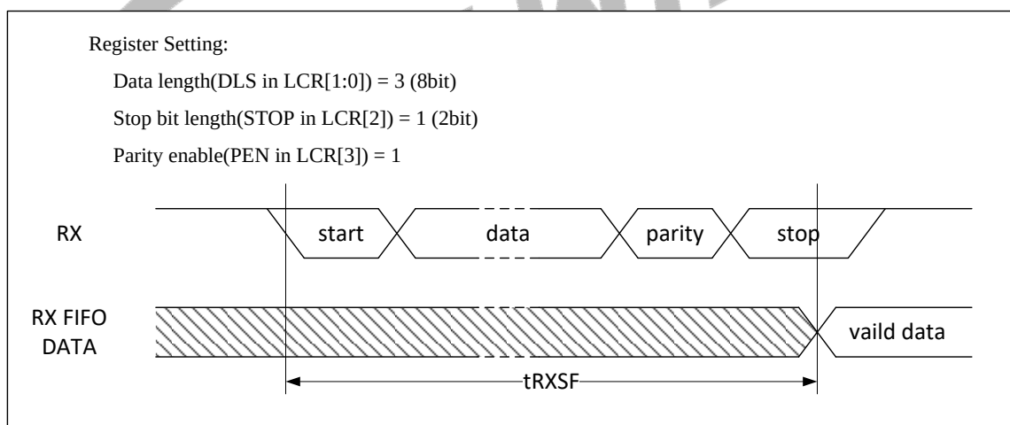
Figure 5-17 UART RX Timing
