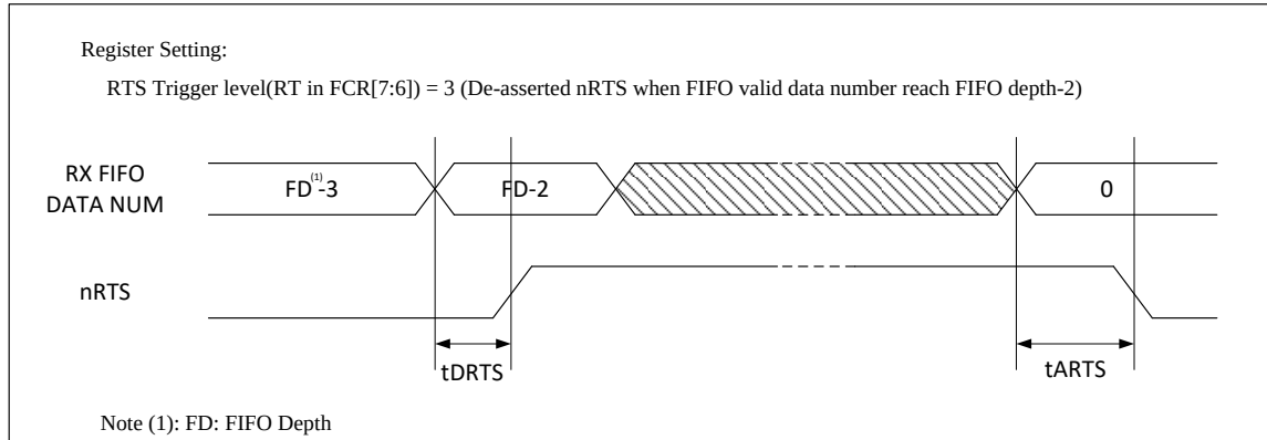
Figure 5-19 UART nRTS Timing
