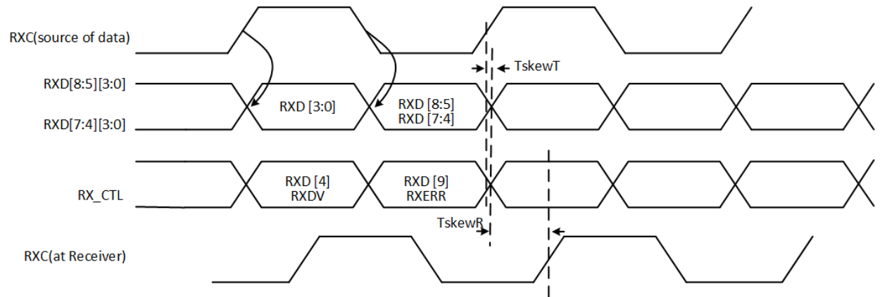
Figure 5-11 RGMII-ID Interface Transmit Timing
