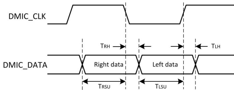
Figure 5-23 DMIC Timing
