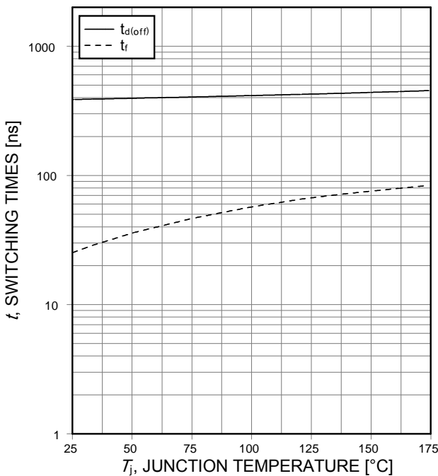
Figure 11. Typical switching times as a function of junction temperature (ind. load, V_{CE}=600\text{V} , V_{GE}=15/0\text{V} , I_C=20\text{A} , R_G=15\Omega , test circuit in Fig. E)
