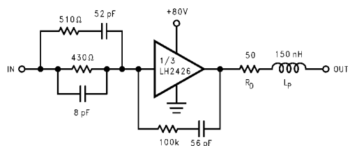
FIGURE 3. One Section of the LH2426 with Damping Resistor R_D and Peaking Inductance L_P in the Output
