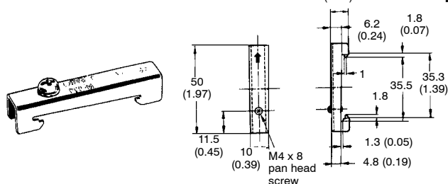
End Plate PFP-M
