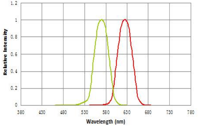
Spectrum Distribution (Ta=25°C)
