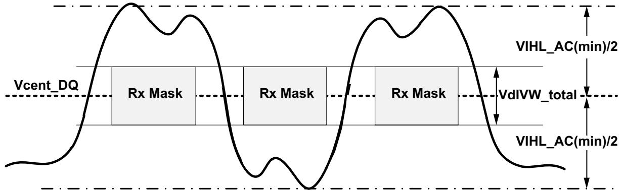
Figure 194 - DQ VIH_L_AC definition (for each input pulse)
