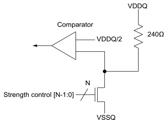
Figure 181 - Pull-down calibration
