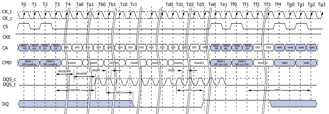
Figure 108 - Write Leveling Timing, tDQSL(min)
