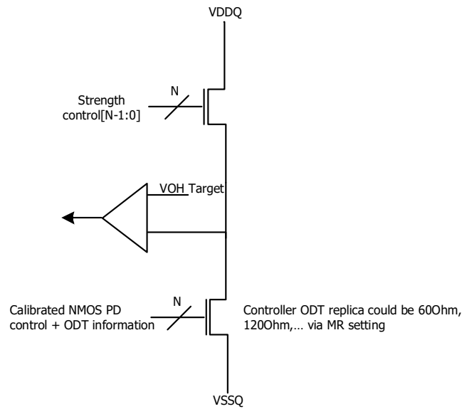
Figure 182 - Pull-up calibration
