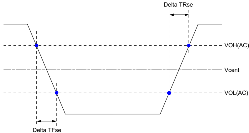
Figure 176 - Single Ended Output Slew Rate Definition
