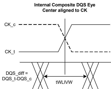
Figure 110 - DQS t /DQS c and CK t /CK c at DRAM Latch
