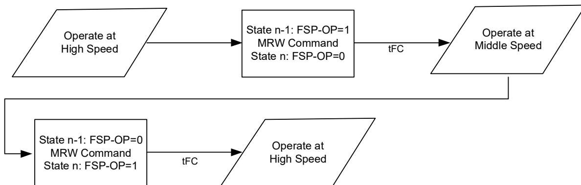
Figure 105 - Switching between two trained Frequency Set Points
