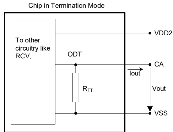
Figure 134 - On Die Termination for CA
