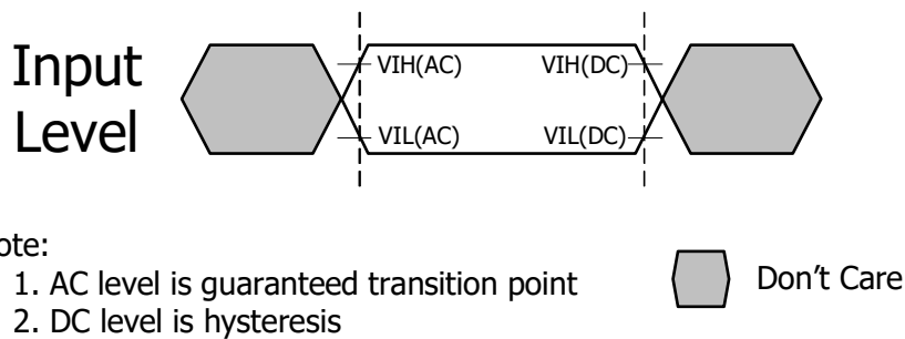
Figure 163 - Input AC timing definition for CKE
