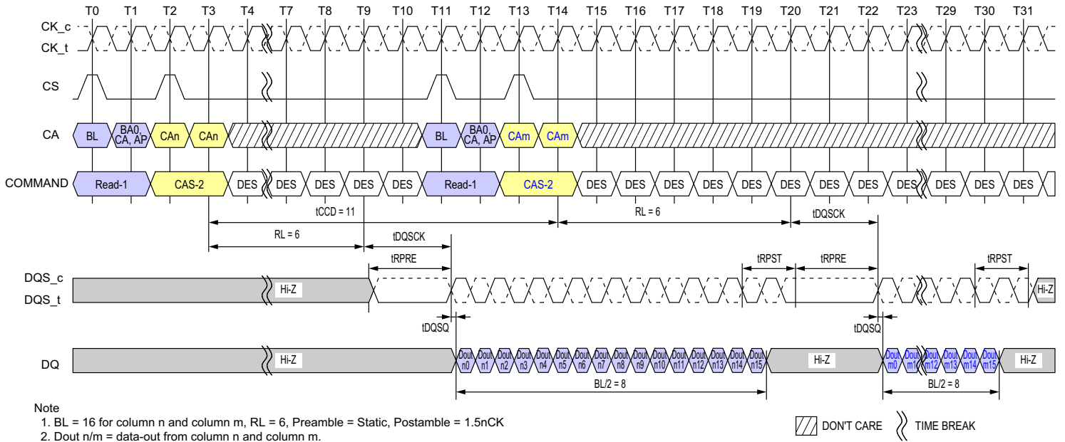
Figure 41 - Consecutive Reads Operation: tCCD = Min +3, Preamble = Static, 1.5nCK Postamble
