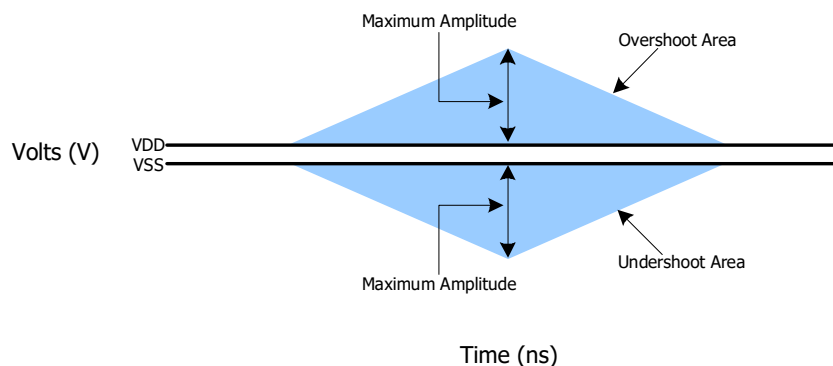
Figure 178 - AC Overshoot and Undershoot Definition
