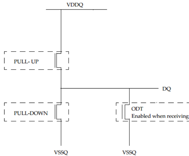
Figure 180 - LVSTL I/O Cell
