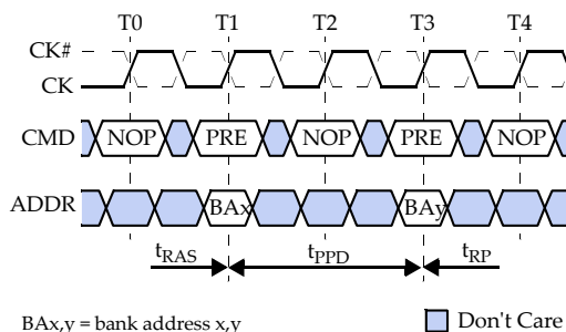
Figure 69. PRECHARGE command
