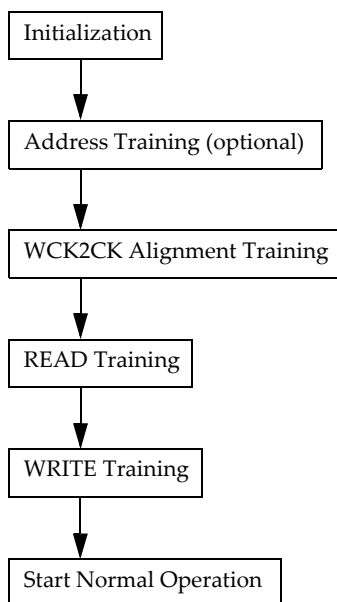
Figure 8: Interface Training Sequence
