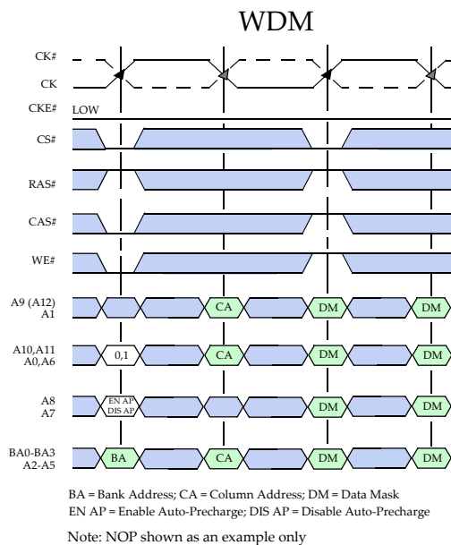
Figure 51. WRITE-With-Doublebyte-Mask Command
