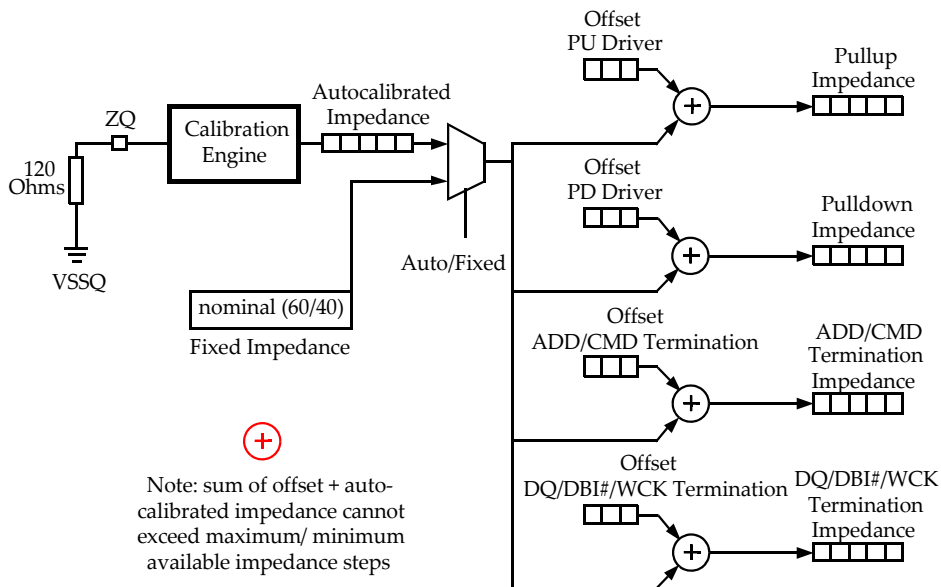
Figure 26. Impedance Offsets
