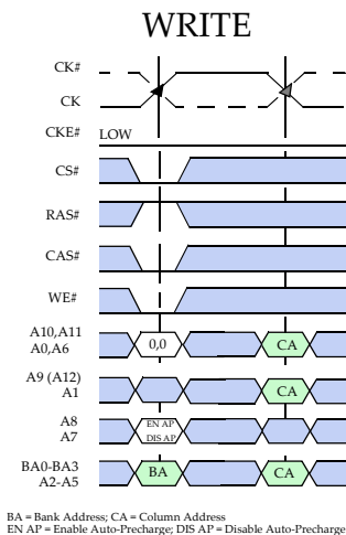
Figure 43. WRITE Command
