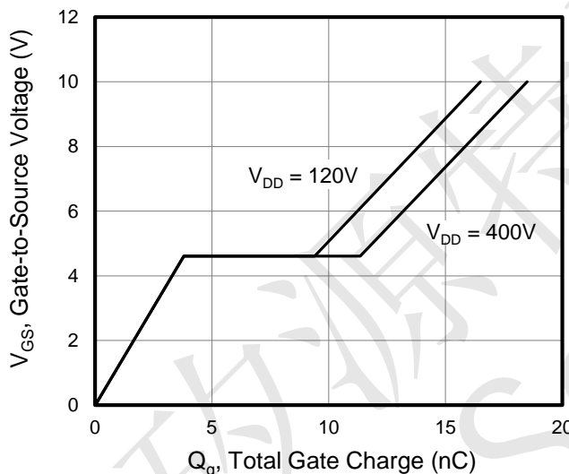
Figure 9. Gate Charge
