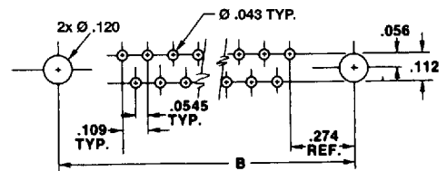
PC BOARD HOLE PATTERN
