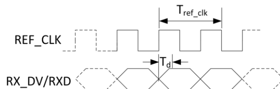
Figure 5-27. RMII Interface Receive Timing
