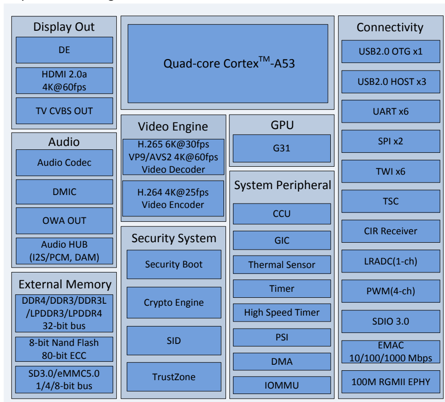
Figure 3-1. H616 System Block Diagram
