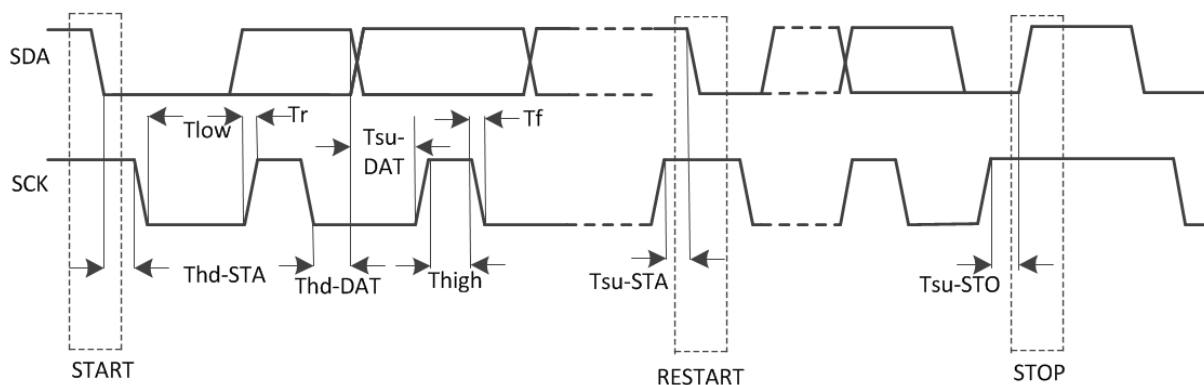
Figure 5-36. TWI Timing
