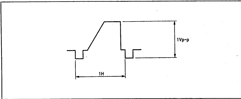
Video Signal-2
