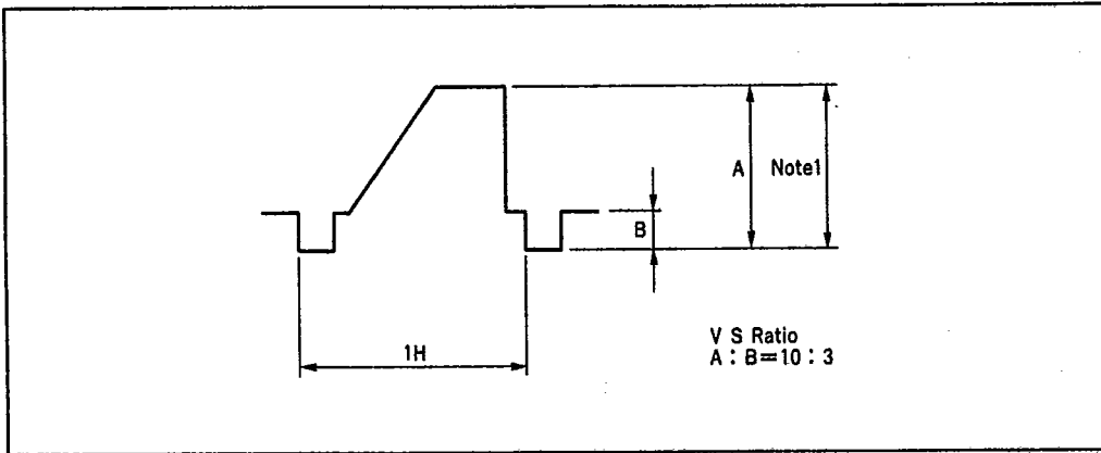
Video Signal-1
