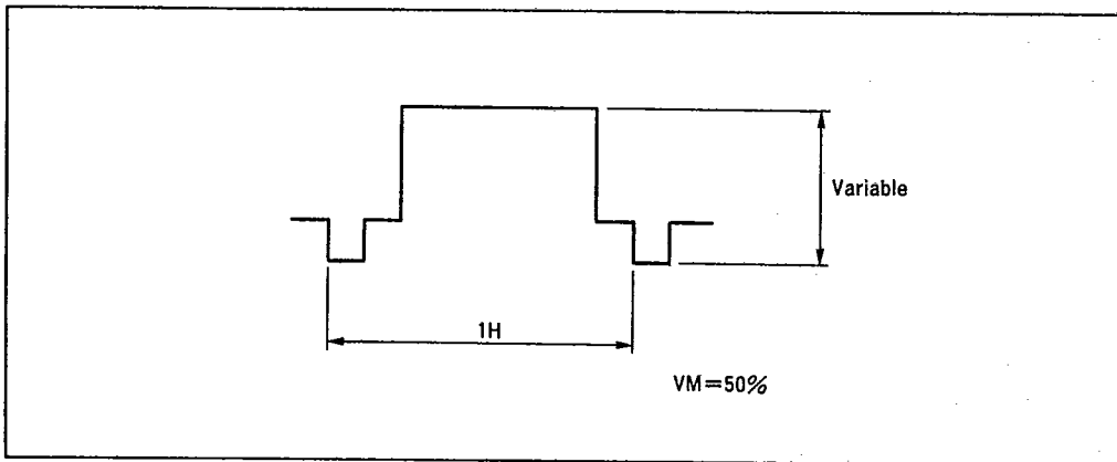
Video Signal-3
