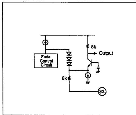
Figure 7. Basic Sync Pulse Adder Circuit
