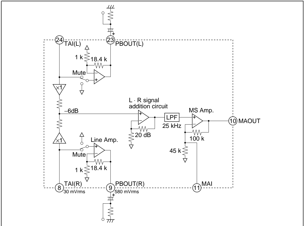
Figure 4 Music Sensor Mixing Amp. Block Diagram
