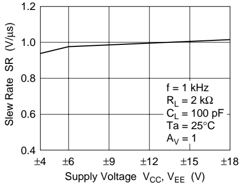
Slew Rate vs. Supply Voltage
