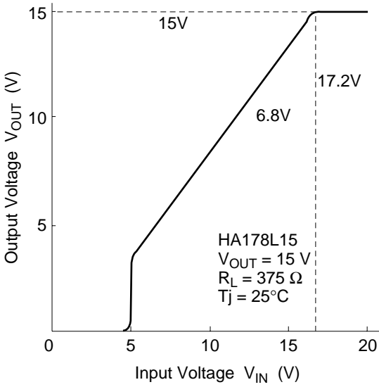
Output Voltage vs. Input Voltage (3)
