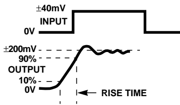
TRANSIENT RESPONSE
