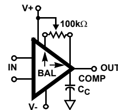
SUGGESTED V_{OS} ADJUSTMENT AND COMPENSATION HOOK-UP
