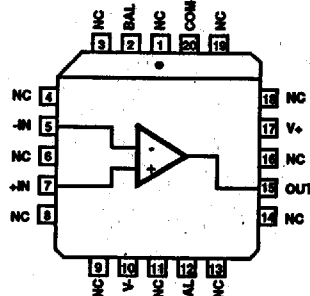
HA-2625, (PLCC) TOP VIEW
