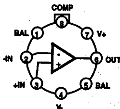
HA-2620, HA-2622, HA-2625 (CAN) TOP VIEW
