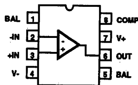
HA-2620/22 (CDIP) HA-2528 (CDIP, PDIP, SOIC) TOP VIEW
