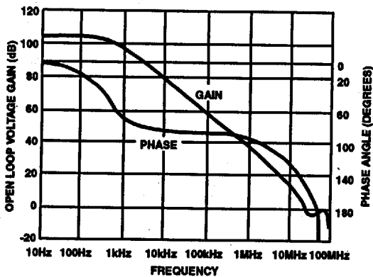
FIGURE 3. OPEN LOOP FREQUENCY AND PHASE RESPONSE
