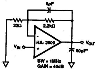
FIGURE 12. VIDEO AMPLIFIER
