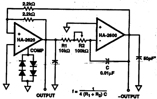
FIGURE 11. FUNCTION GENERATOR
