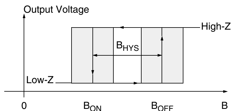
Fig. 4–15: Definition of magnetic switching points for the HAL 1510
