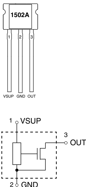
Fig. 4–5: Pin configuration
