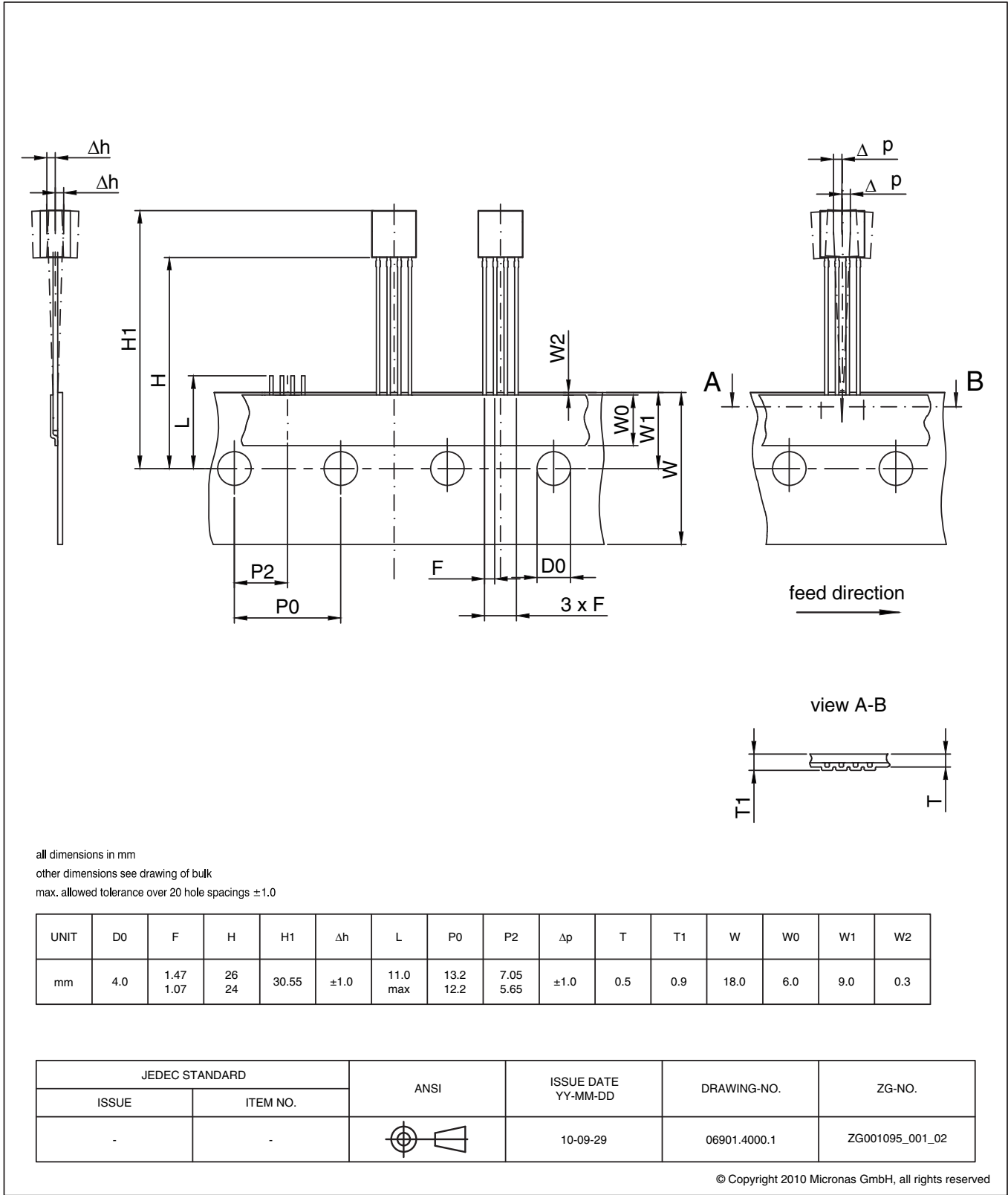
Fig. 4-3: T092UP : Dimensions ammpack inline, not spread
