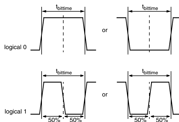
Fig. 6–1: Definition of logical 0 and 1 bit
