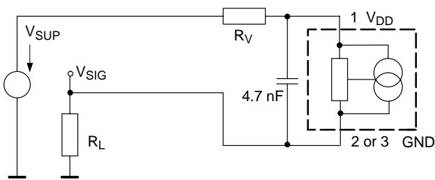
Fig. 5–2: Application Circuit 2
