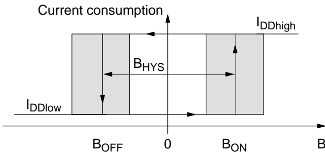
Fig. 1-3: Latching Sensor
