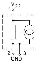
Fig. 1-4: Pin configuration
