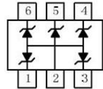
Pin Configuration
