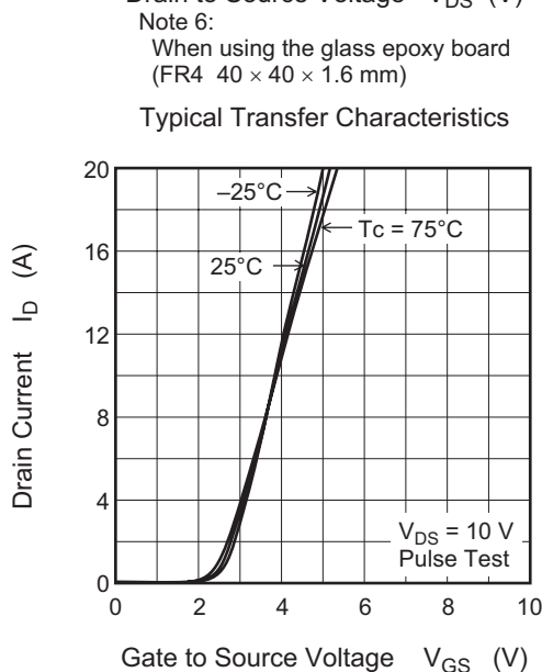
Typical Transfer Characteristics
