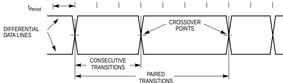
Figure 10-14. Data Jitter
