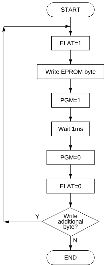
Figure A-2. EPROM Programming Sequence
