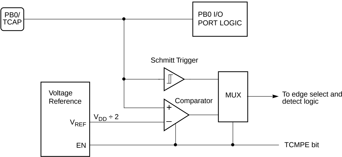
Figure 9-7. TCAP Input Signal Conditioning
