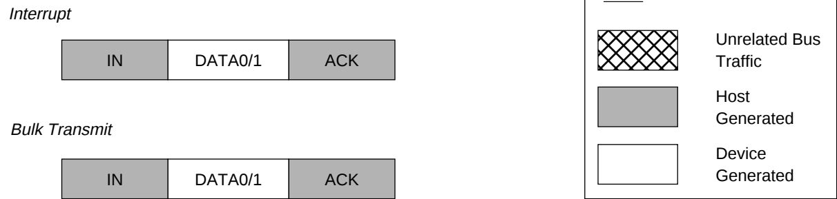
Figure 10-2. Supported Transaction Types per Endpoint
