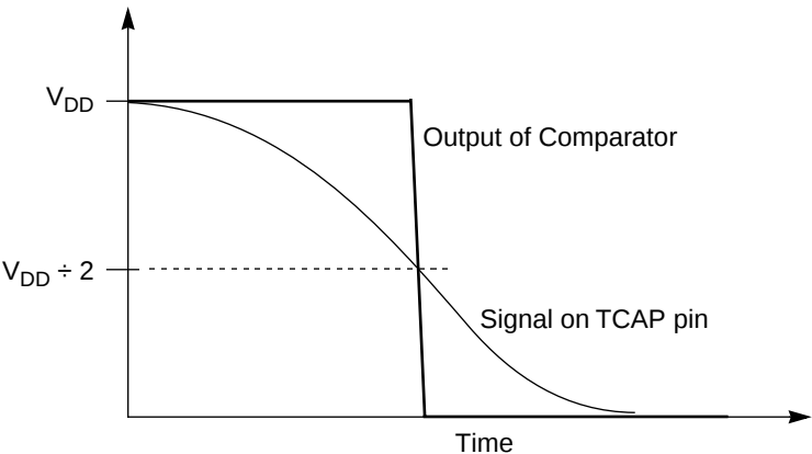
Figure 9-8. TCAP Input Comparator Output
