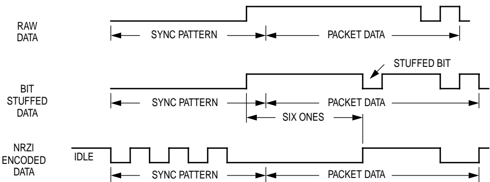
Figure 10-18. Bit Stuffing
