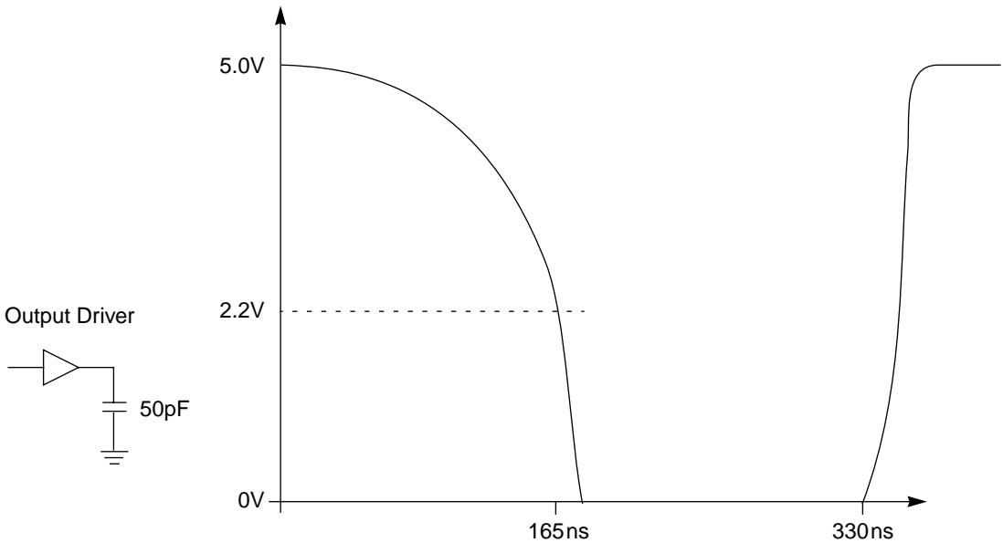
Figure 7-1. Slow Falling-edge Output Driver
