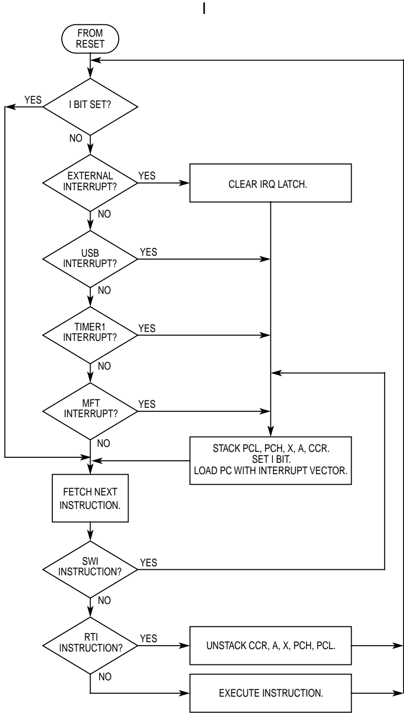
Figure 4-2. Interrupt Flowchart
