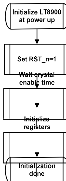
Figure 6. Initialization flowchart
