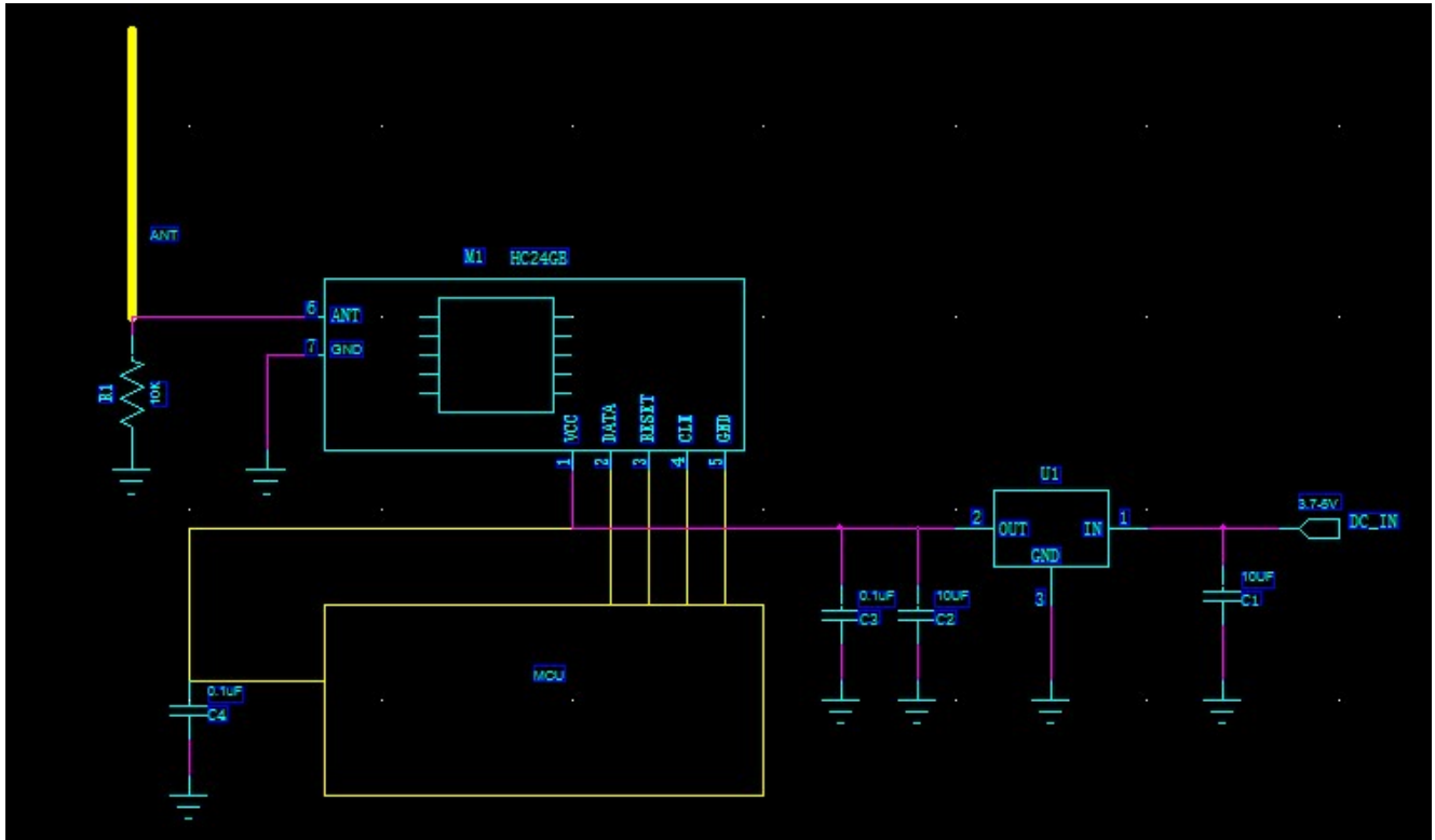
Figure 1. HC24GB Typical Application Schematic
