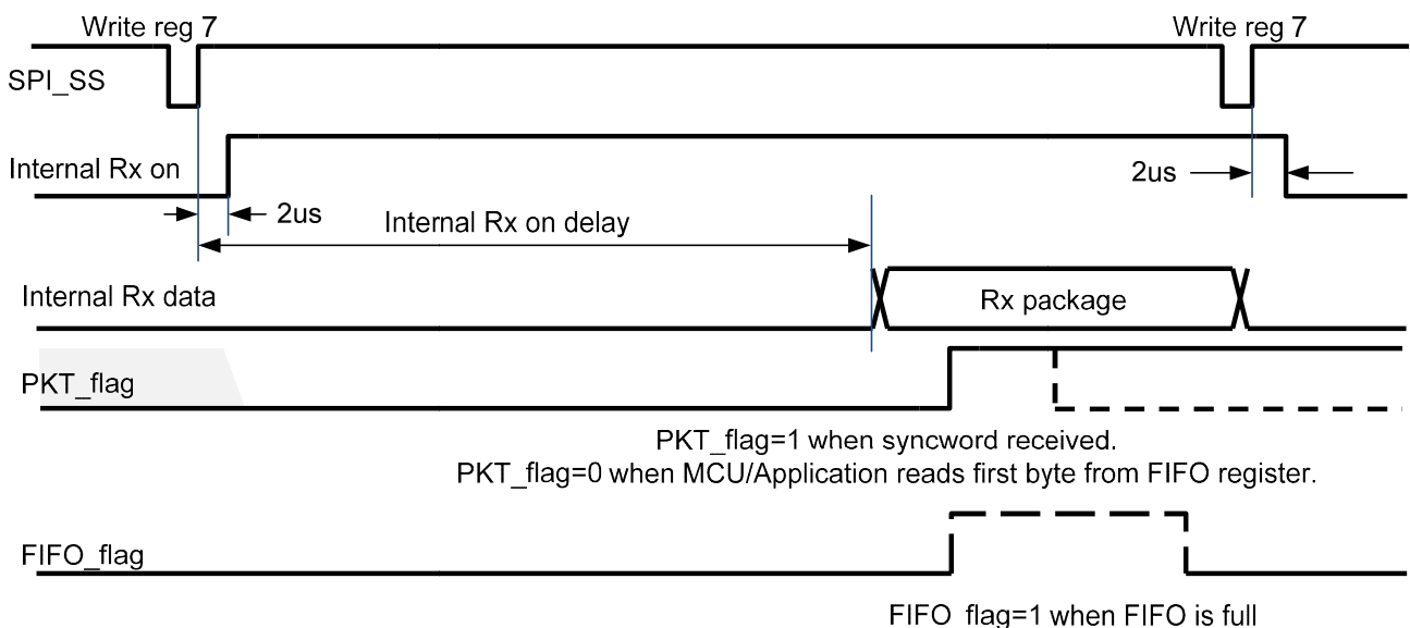
Figure 15. RX timing diagram when Register 41[13:12] = 'b00 or 'b01.
