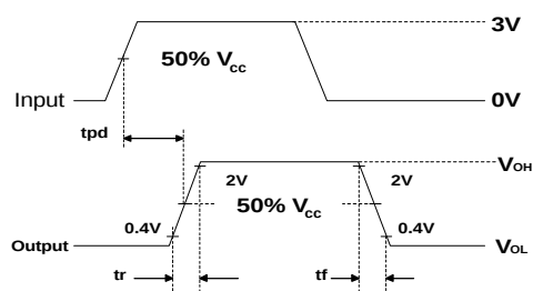
Voltage Waveforms
