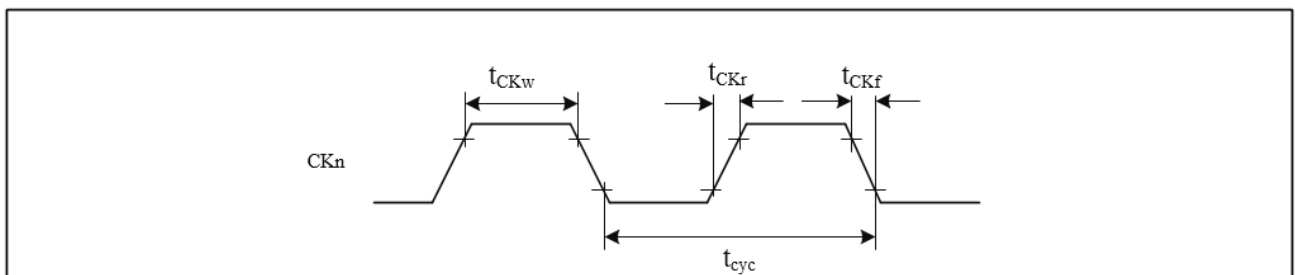
Figure 3-23 USART clock timing
