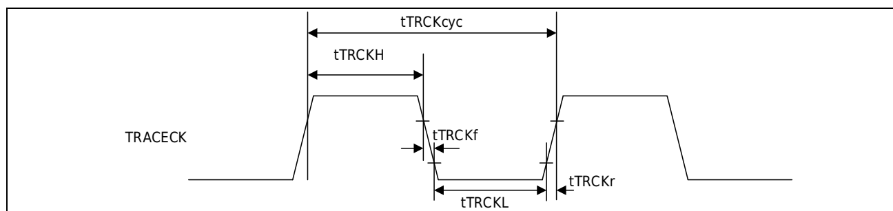
Figure 3-29 TRACE clock
