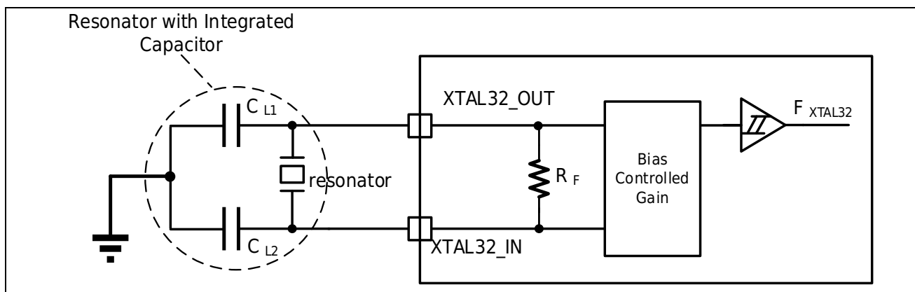
Figure 3-5 Typical Application Using a 32.768 kHz Crystal
