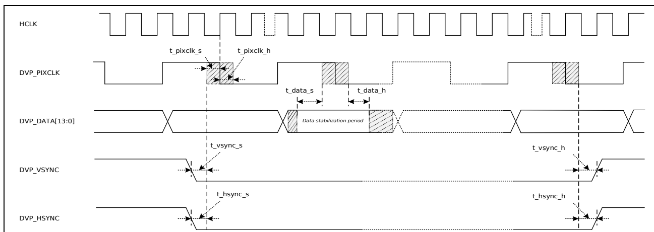
Figure 3-36 DVP input signal timing diagram
