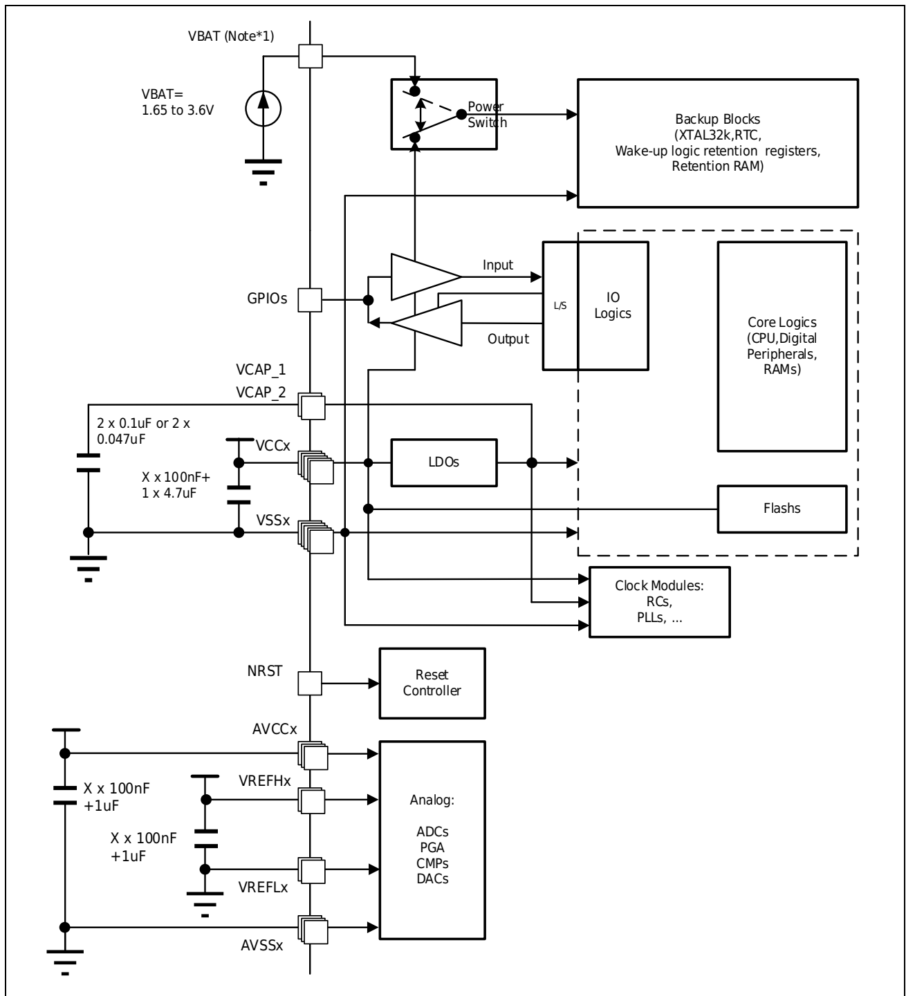
Figure 3-2 Power scheme
