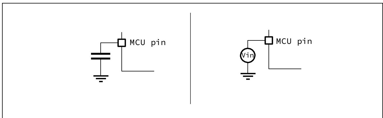
Figure 3-1 Pin Load Condition (Left) vs Input Voltage Measurement (right)
