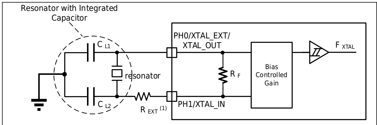
Figure 3-4 Typical Application Using an 8 MHz Crystal
