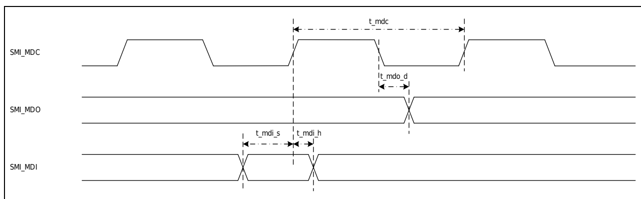
Figure 3-19 ETHMAC-SMI interface timing diagram
