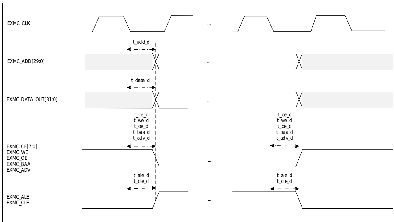
Figure 3-34 EXMC output signal timing diagram
