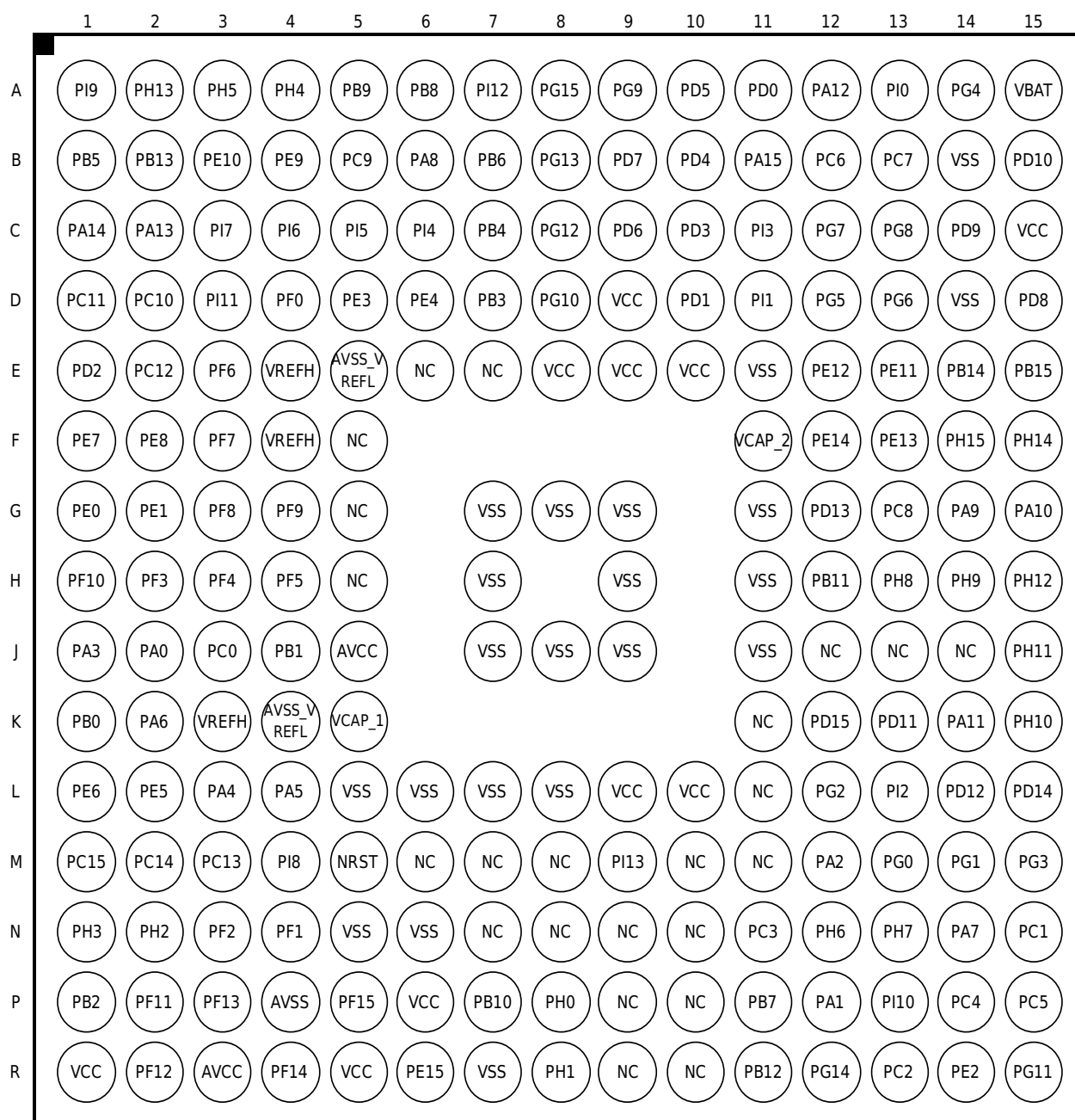
Figure 2-1 Pin configuration diagram
