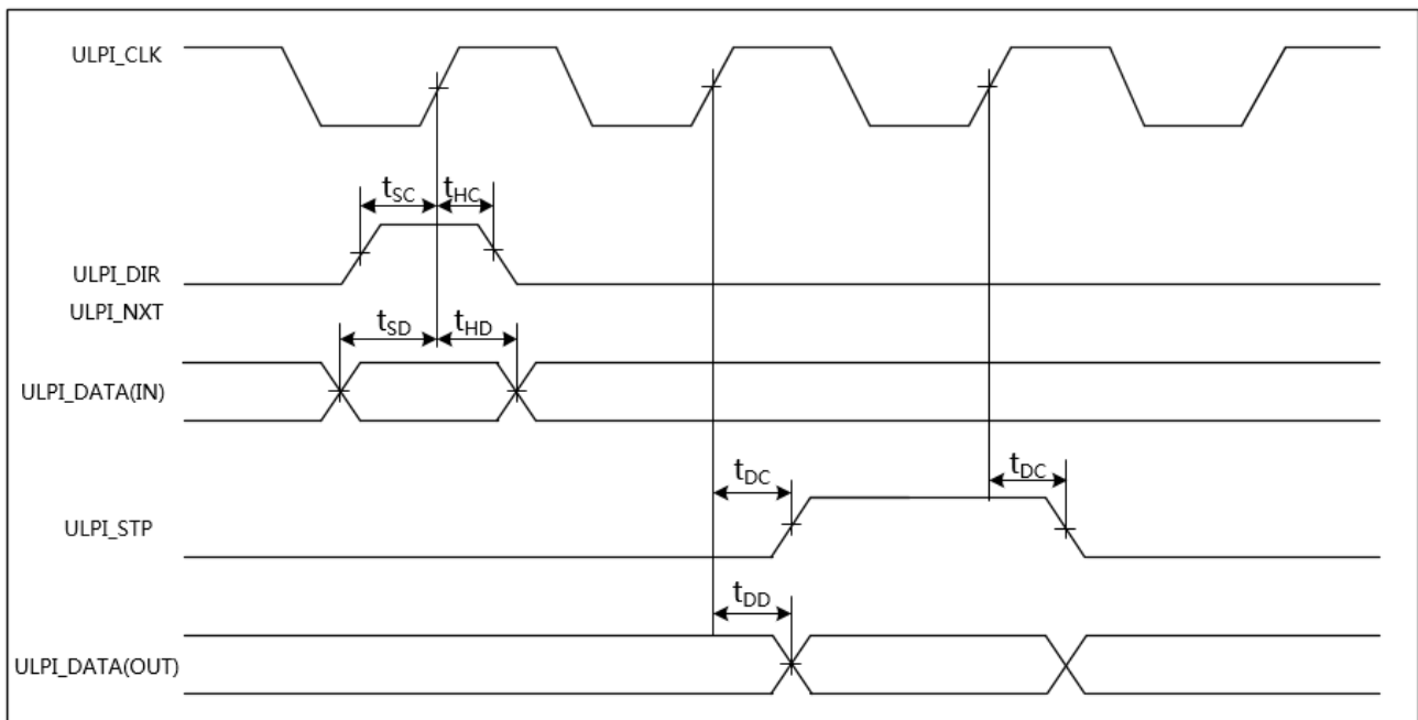
Figure 3-18 ULPI Timing Diagram
