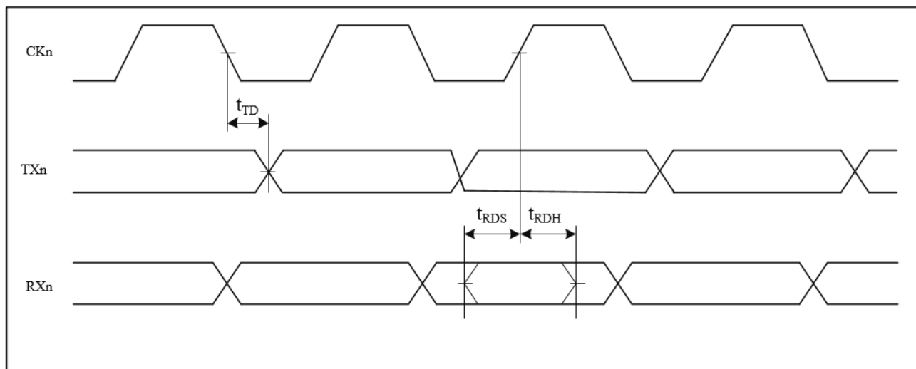
Figure 3-24 USART (CSI) input and output timing
