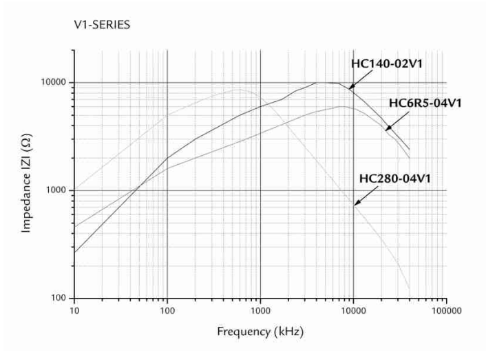
Curves: Impedance vs. Frequency
