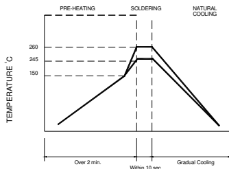
Figure 2. Wave Soldering
