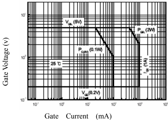
FIGURE 1 – Gate Characteristics
