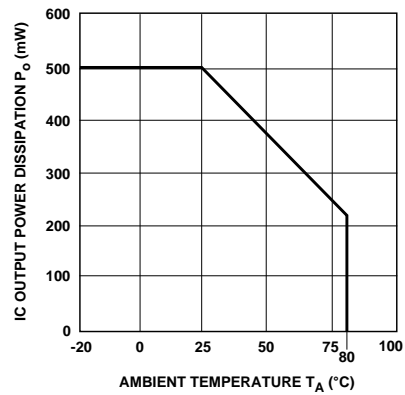
Figure 10. Maximum IC Output Power Dissipation vs. Ambient Temperature.
