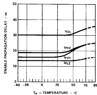
Figure 10. Typical Enable Propagation Delay vs. Ambient Temperature.
