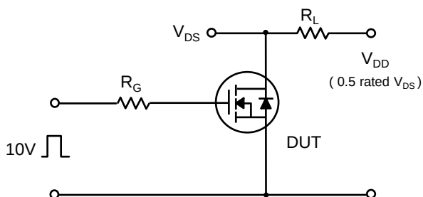
Fig 13. Resistive Switching Test Circuit &amp; Waveforms
