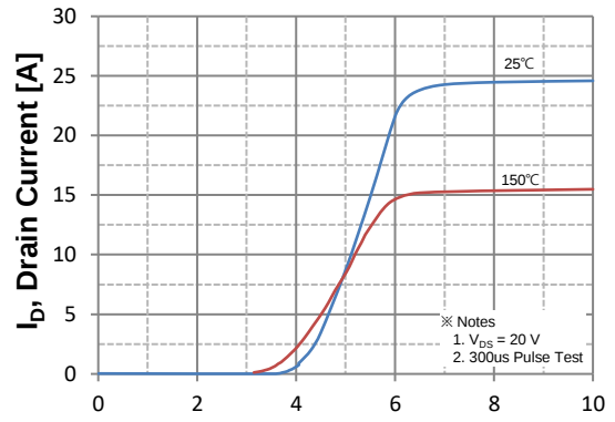
Figure 2. Transfer Characteristics
