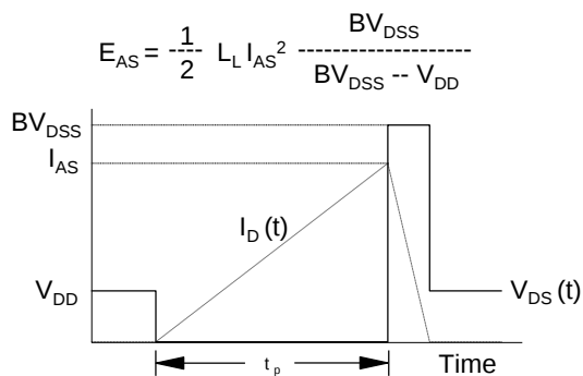
Fig 14. Unclamped Inductive Switching Test Circuit &amp; Waveforms
