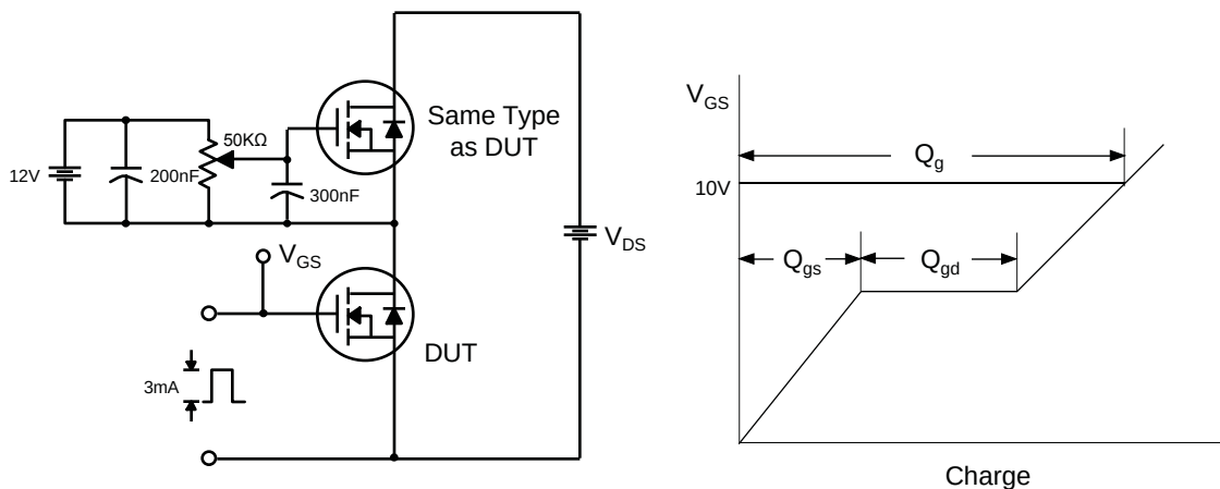
Fig 12. Gate Charge Test Circuit &amp; Waveform
