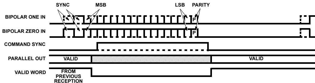
FIGURE 5. DECODER TIMING
