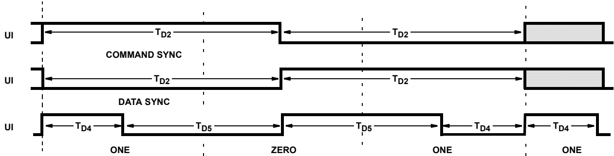
FIGURE 11. DECODER TIMING
