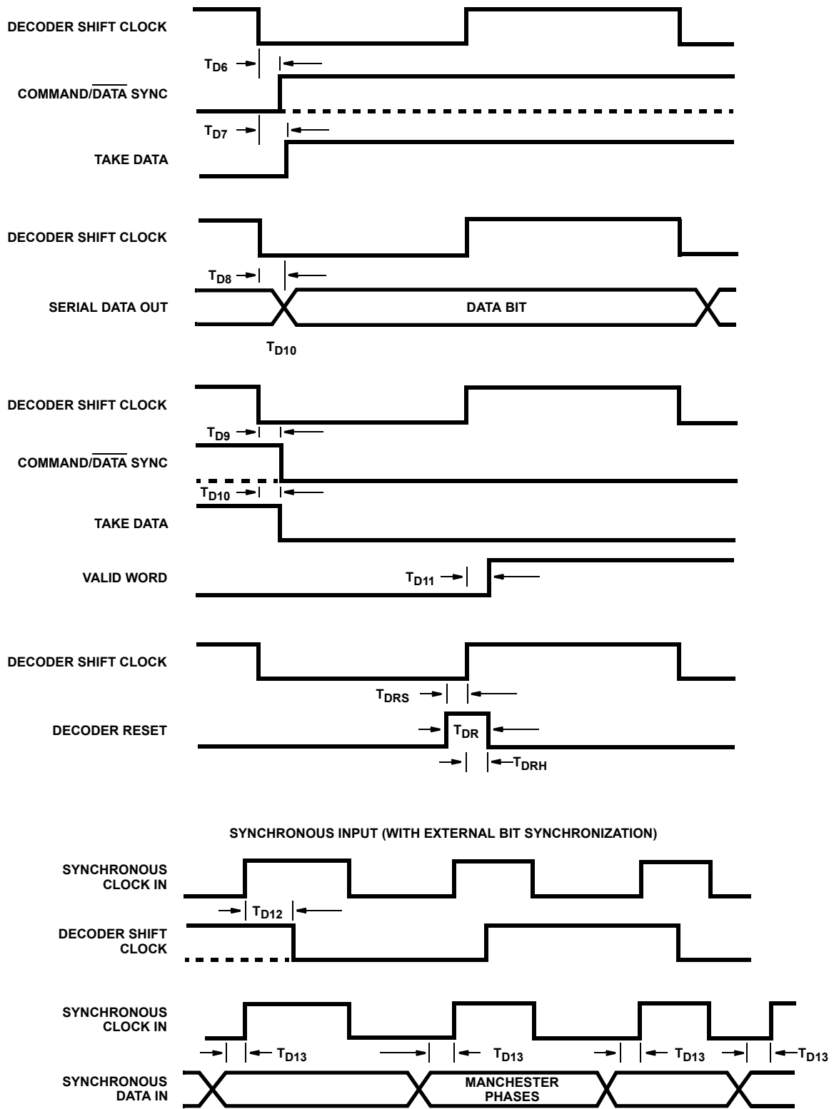
FIGURE 12. DECODER TIMINGS
