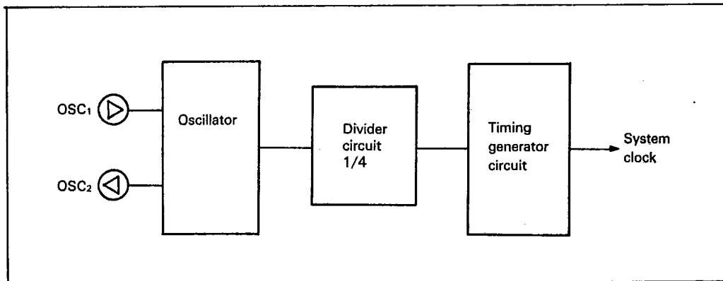
Figure 16. Internal Oscillator Circuit
